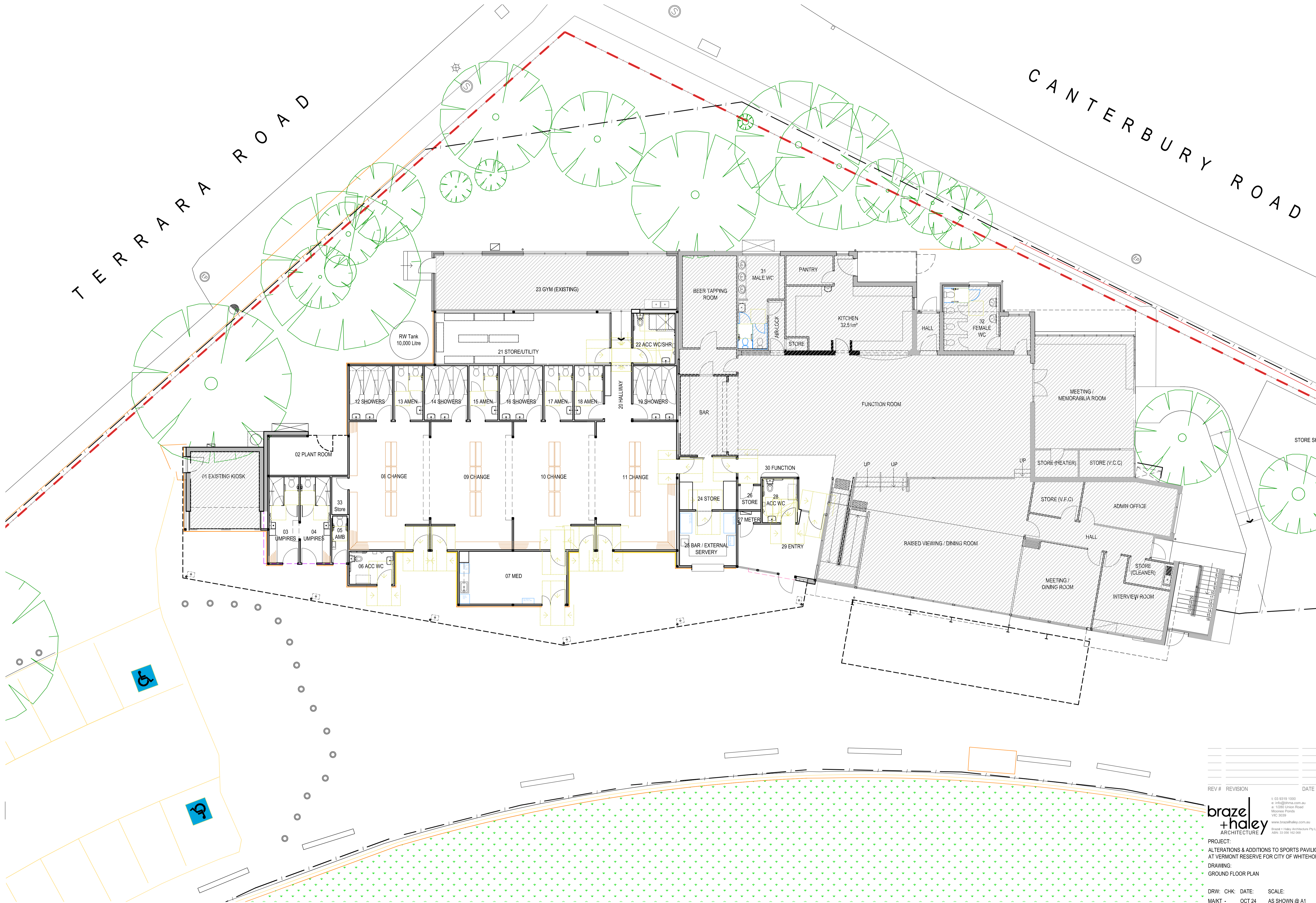
GROUND FLOOR PLAN 1: 100 @ A1
